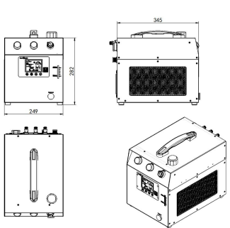
Water Chiller
